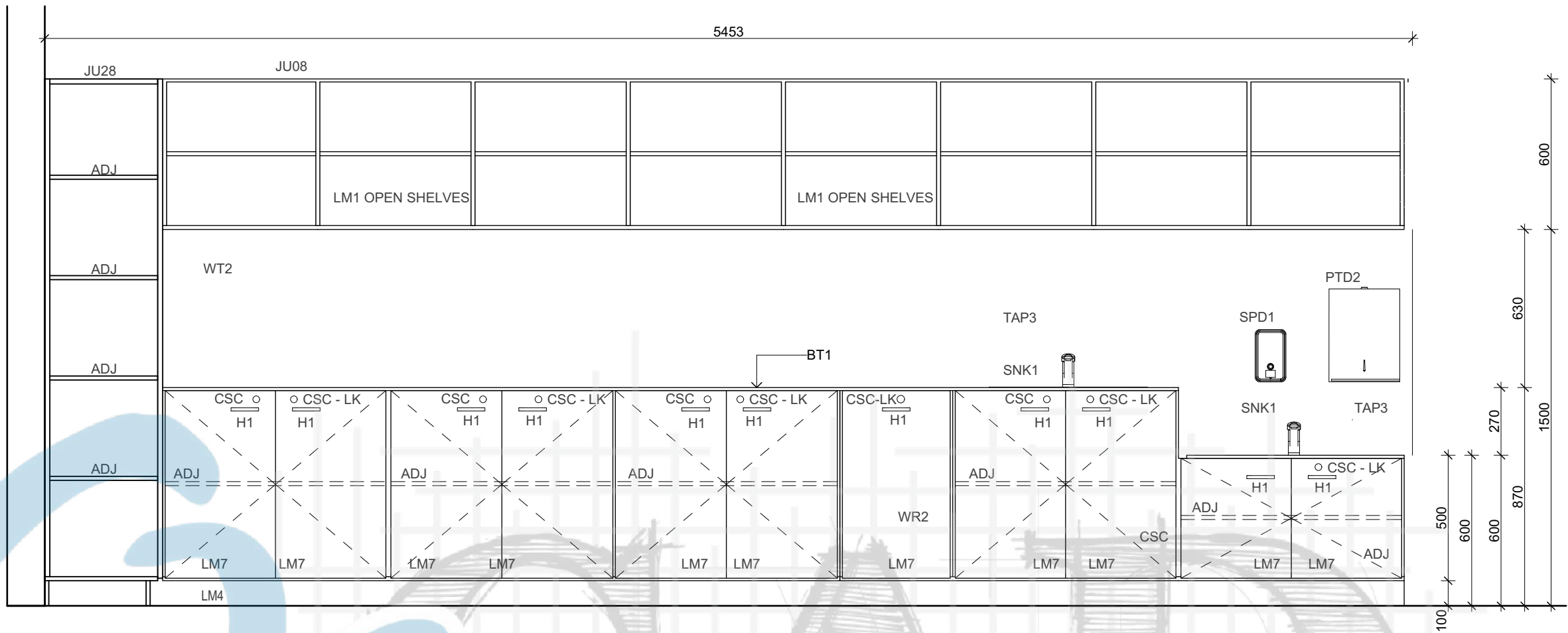
08-E1 FRONT ELEVATION 1:20
