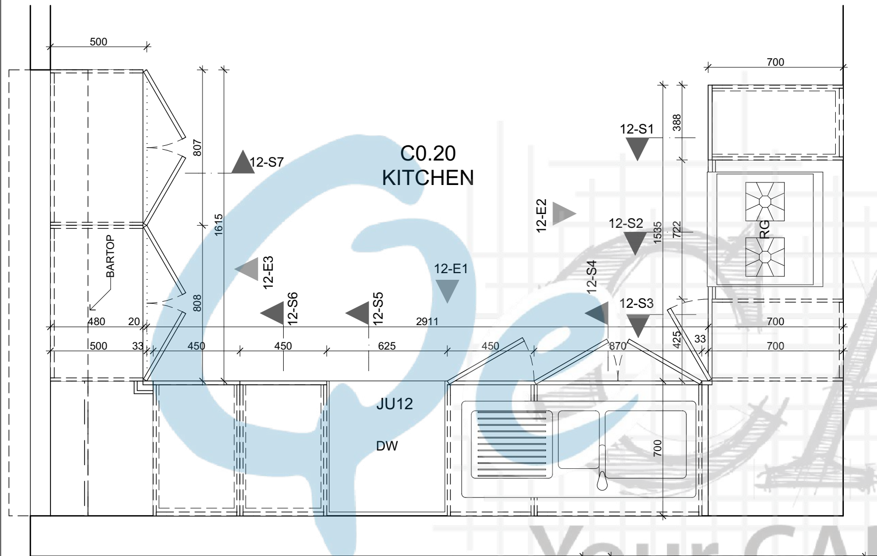
JU12 PLAN 1:20
