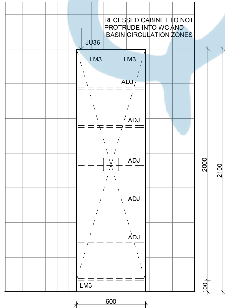
36-E1 FRONT ELEVATION 1:20
