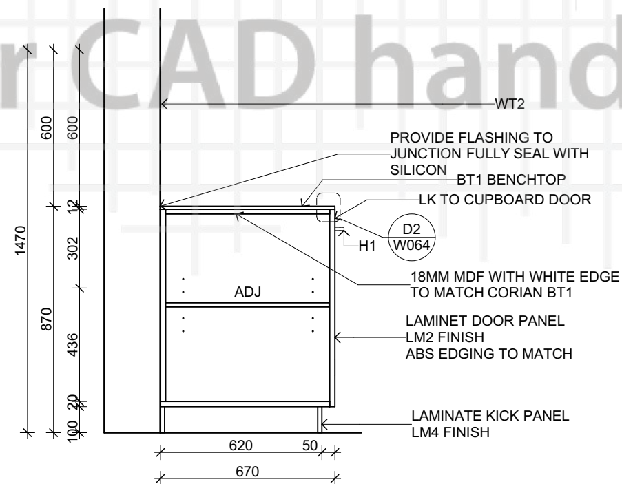
04-S2 Section
