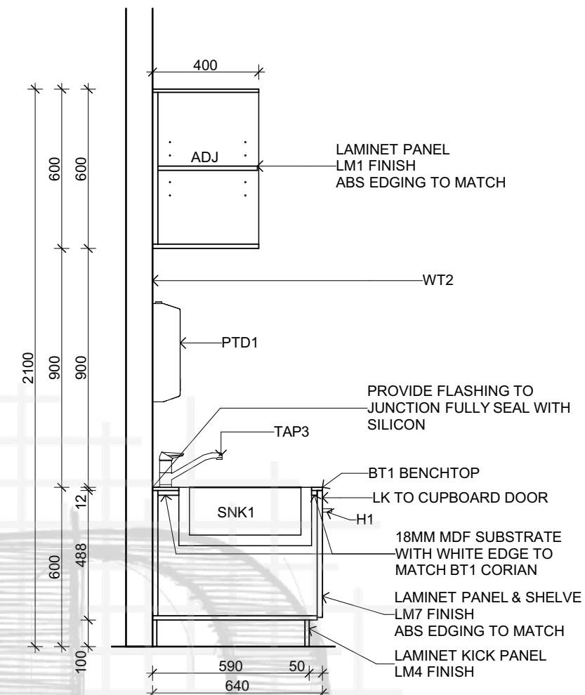
08-S4 Section
