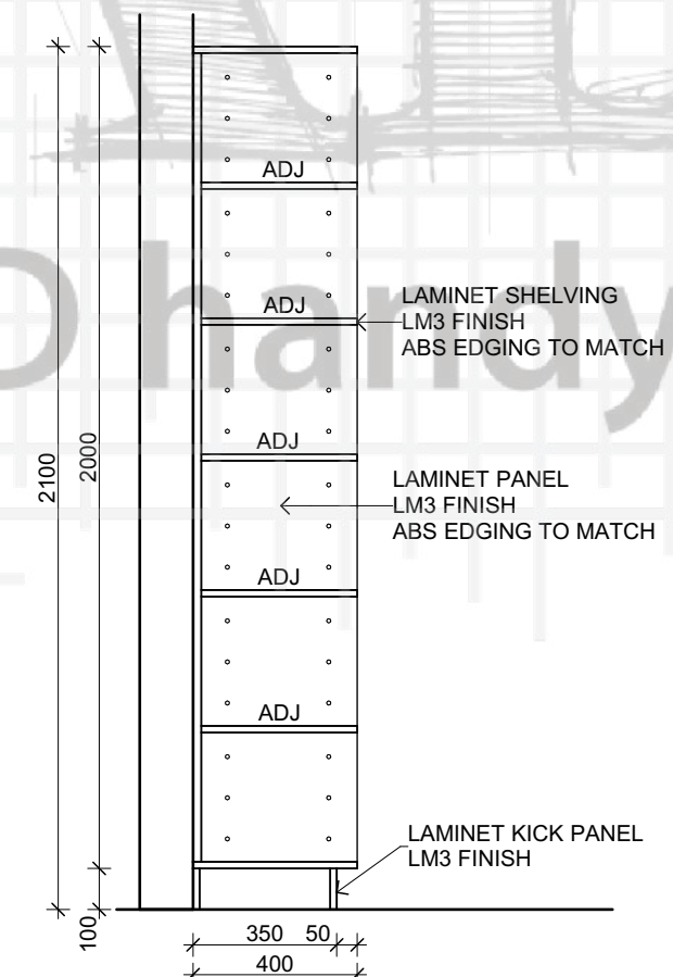
05-S1 Section
