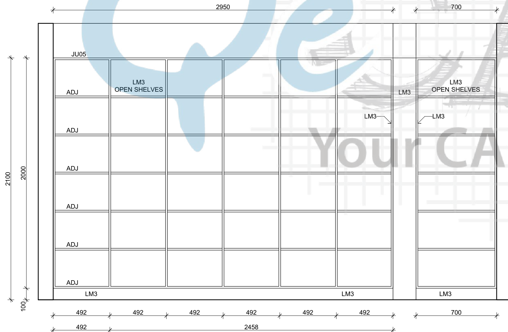
05-E1 FRONT ELEVATION 1:20
