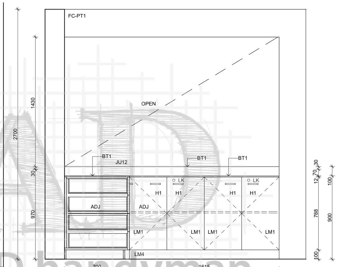
12-E3 FRONT ELEVATION 1:20
