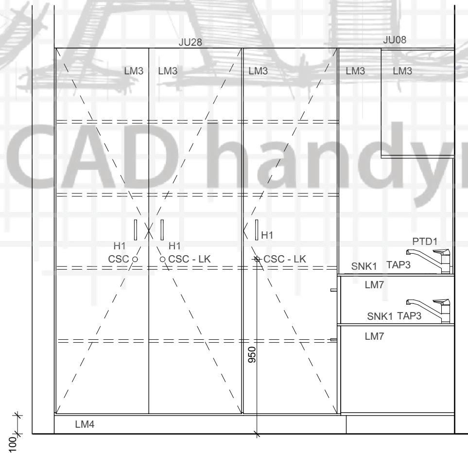
28-E1 FRONT ELEVATION 1:20
