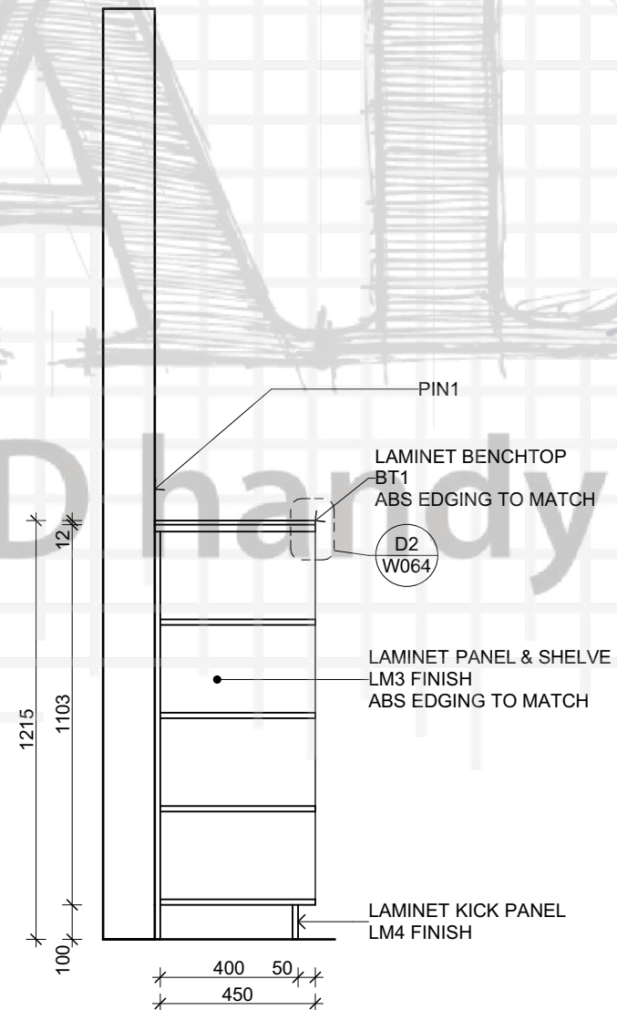
07-S1 Section
