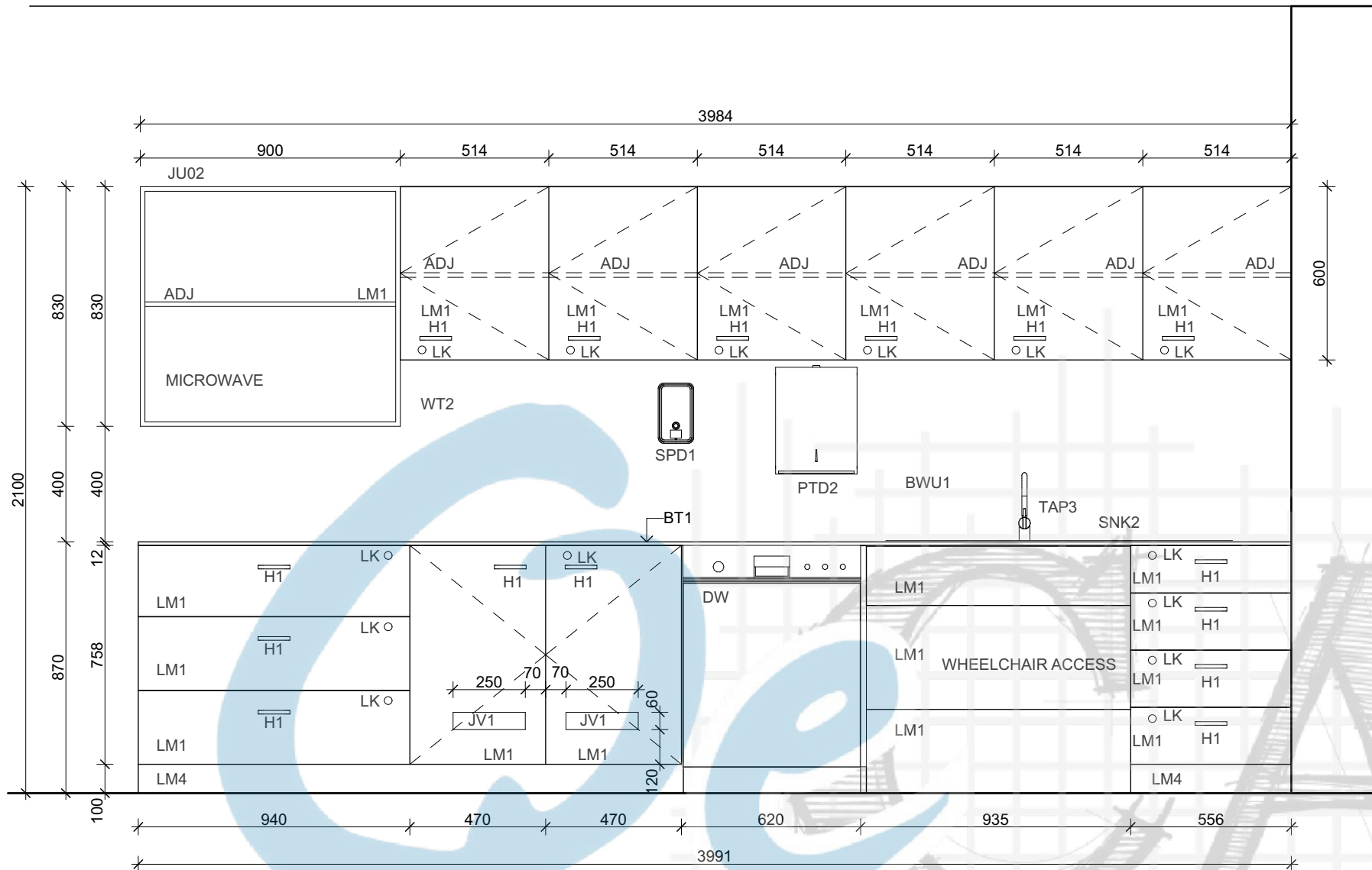
02-E1 FRONT ELEVATION 1:20
