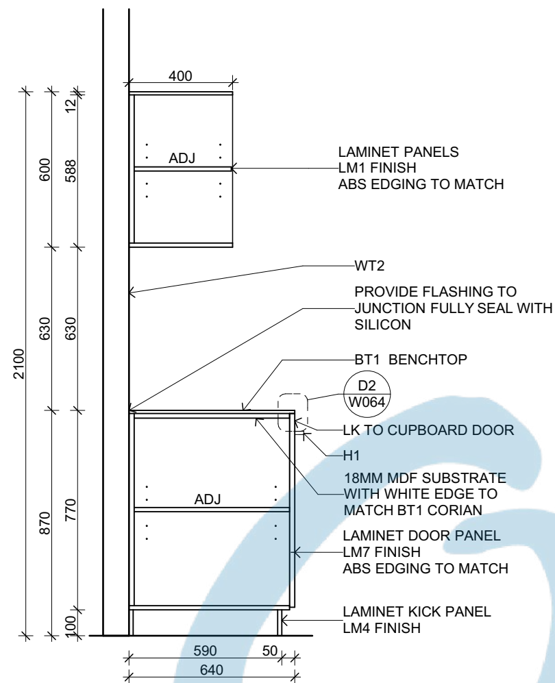
08-S1 Section
