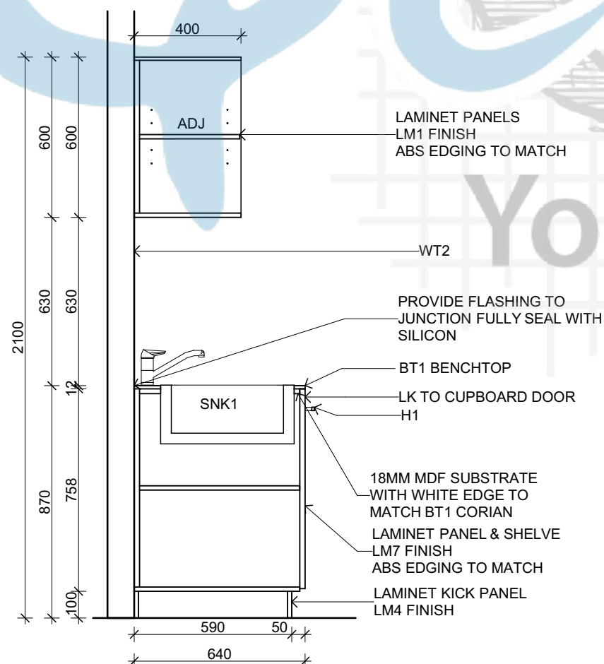
08-S3 Section
