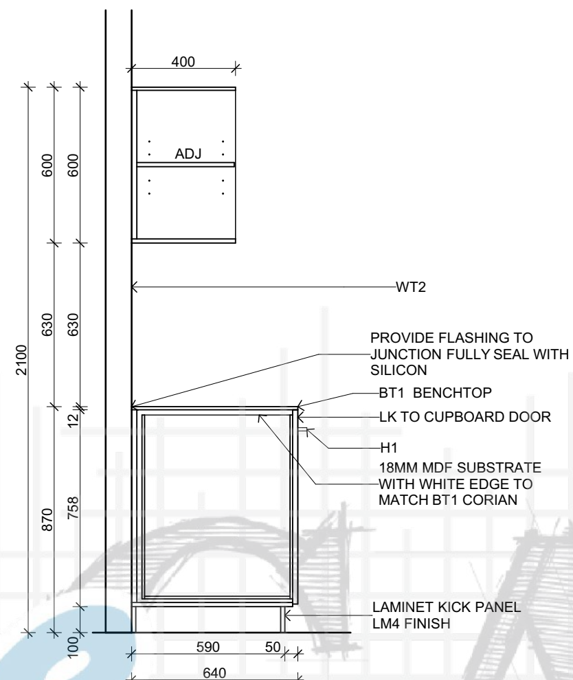
08-S2 Section
